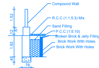
RAIN WATER HARVEST DETAILS
