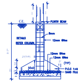
FOUNDATION DETAILS SCALE : 1:50.
