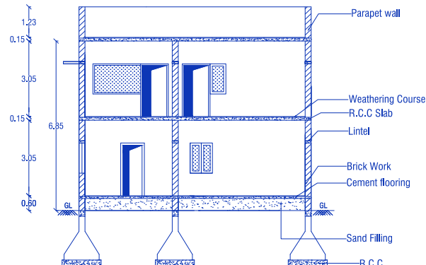
CROSS SECTION ON 'AB'
