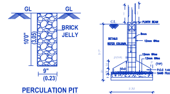
FOUNDATION DETAILS SCALE : 1:50.
