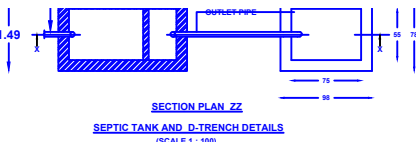
SEPTIC TANK AND D-TRENCH DETAILS (SCALE 1:100)
