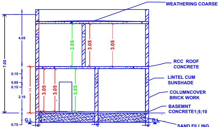
SECTION AB
