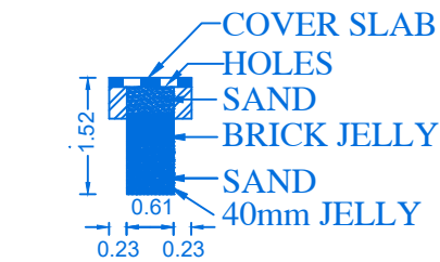
SECTION OF RAIN WATER COLLECTION TANK
