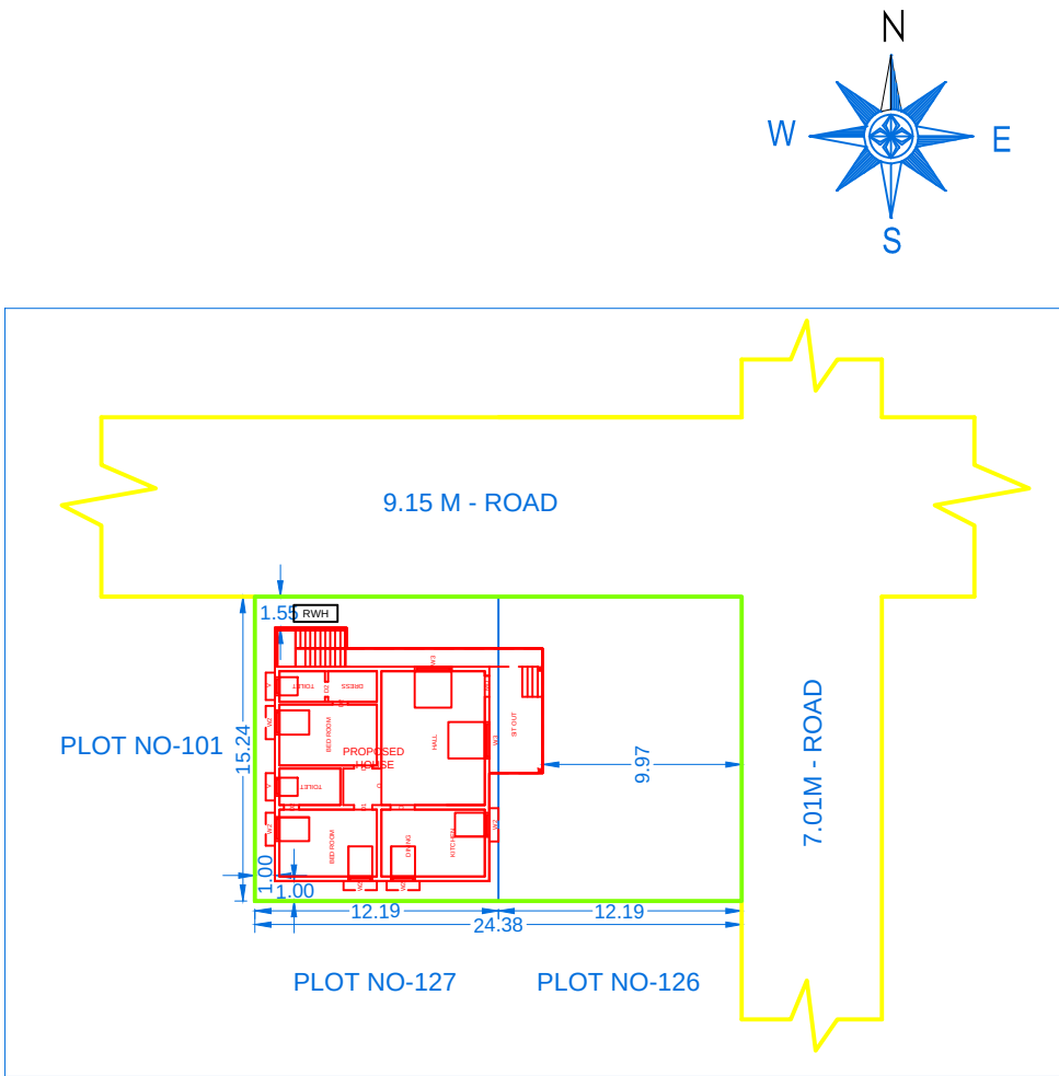
LOCATION PLAN
