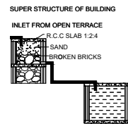
RAINWATER HARVESTING
