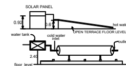
Details of solar water heating system
