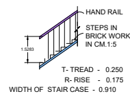
DETAILS OF STAIRCASE
