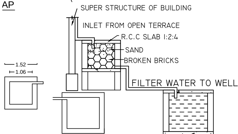
DETAILS OF FILTER BED & WELL RAINWATER HARVESTING
