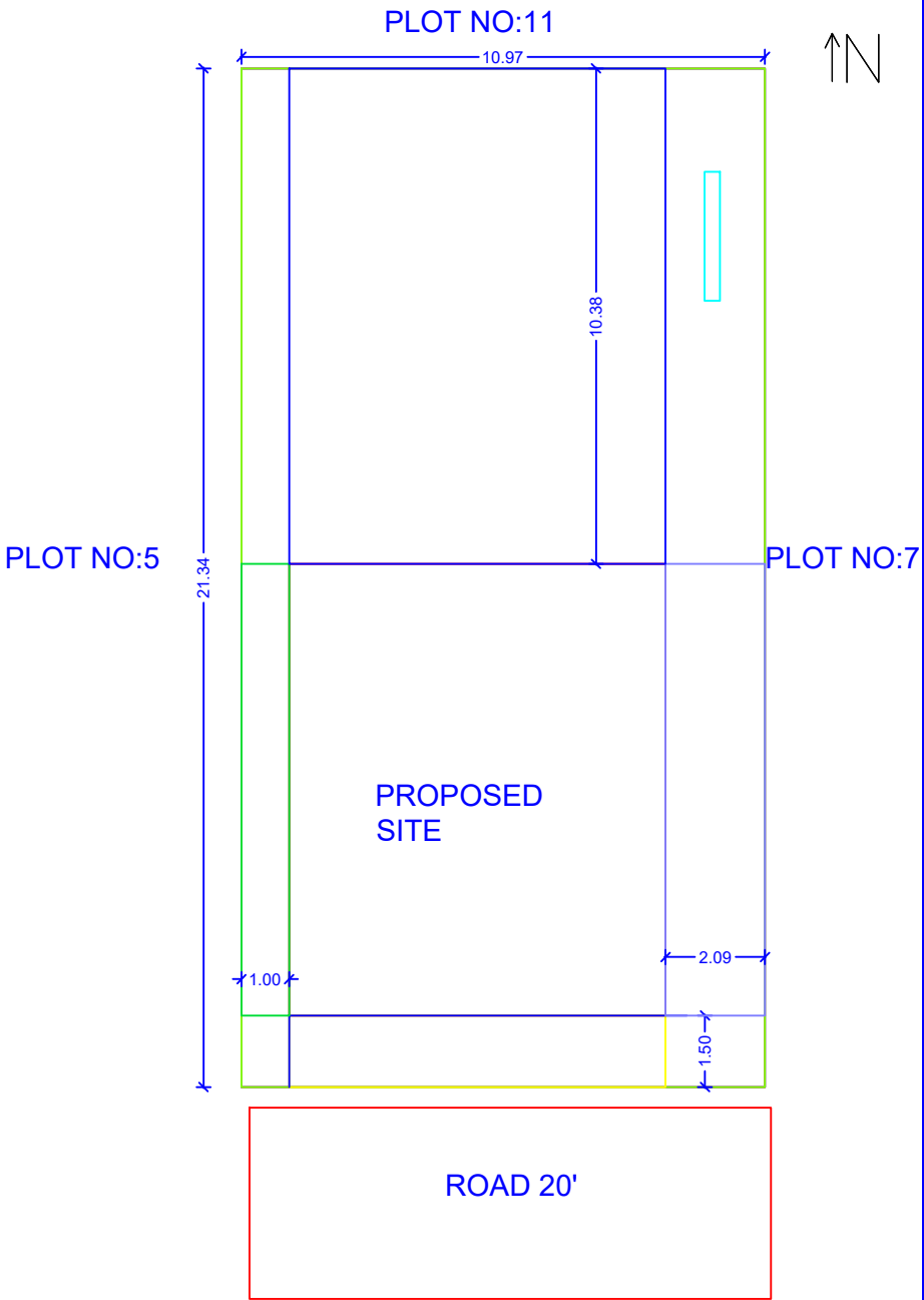
SITE PLAN
