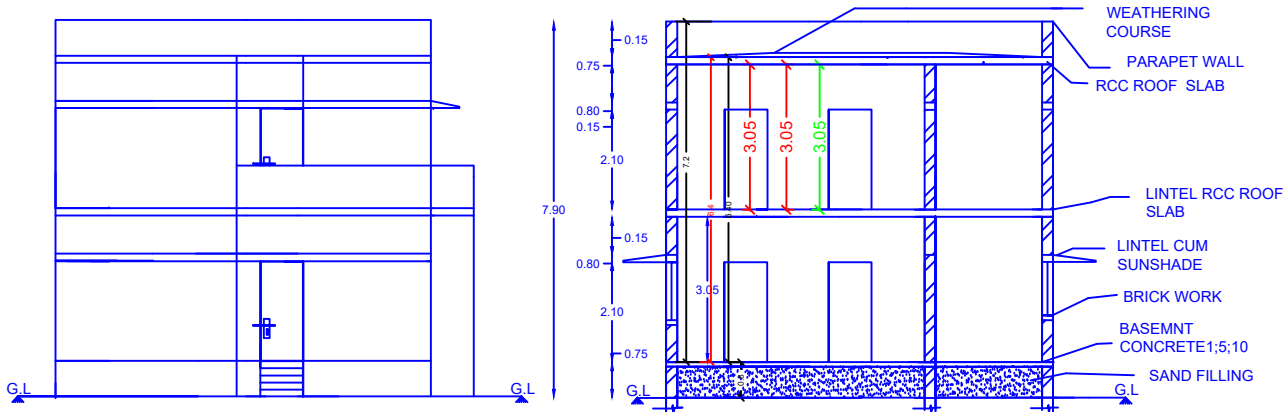
SECTION AB
