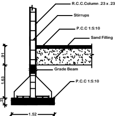
COLUMN DETAIL
