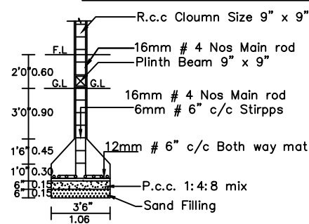
COLUMN DETAIL NOT TO SCALE
