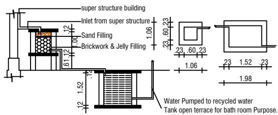
DETAIL PLAN FOR FILTER MEDIA & SUMP
