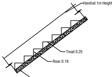
STAIR DETAILS
