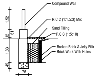
RAIN WATER HARVEST DETAILS
