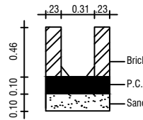
DETAILS OF DRAINAGE PIT
