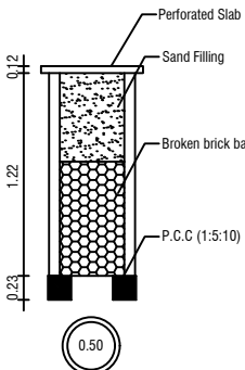
RAIN WATER COLLECTION WELL
