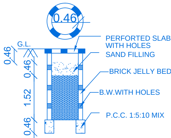
PERCOLATION PIT
