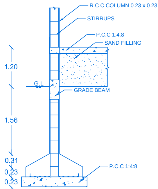
COLUMN DETAIL (SCALE 1:50)
