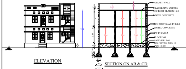
SECTION ON AB & CD
