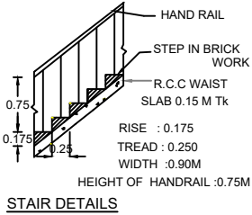
STAIR DETAILS
