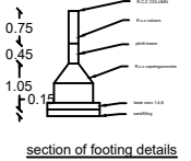
section of footing details
