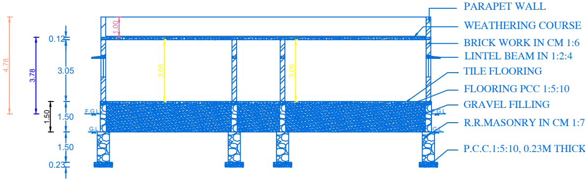
SECTION ON "V-B"
