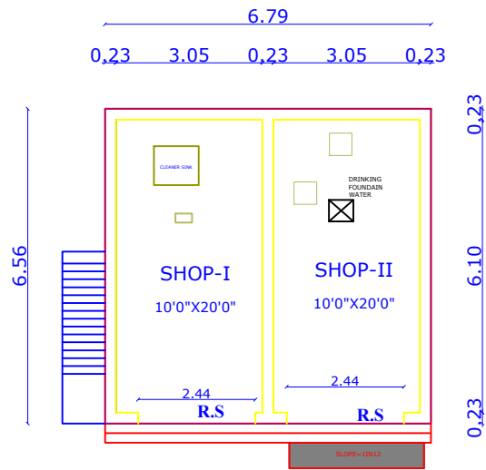
PROPOSED GROUND FLOOR PLAN SHOP (I-II)
