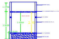
SECTION ON WALL
