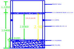
SECTION ON WALL
