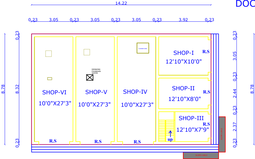
PROPOSED GROUND FLOOR PLAN SHOPS (I-VI)
