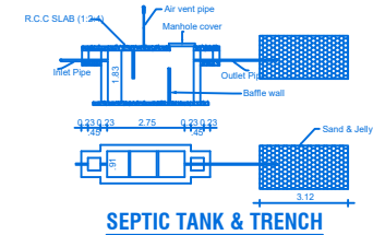
SEPTIC TANK & TRENCH
