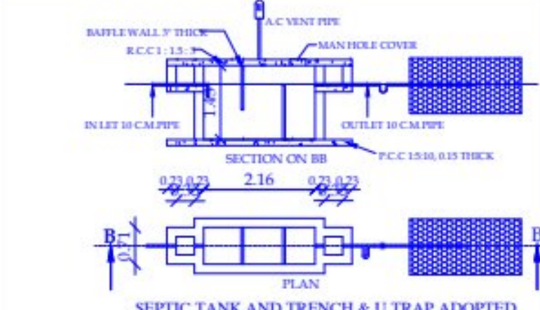
SEPTIC TANK AND TRENCH & U TRAP ADOPTED
