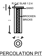
PERCOLATION PIT
