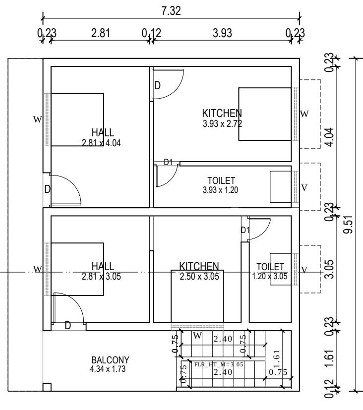
FF PLAN
