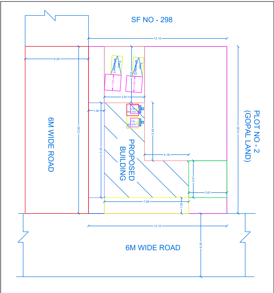
SITE PLAN
