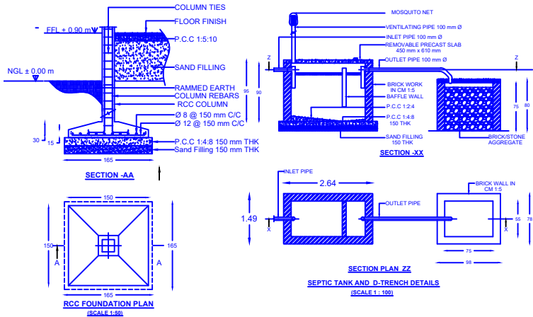
RCC FOUNDATION PLAN
