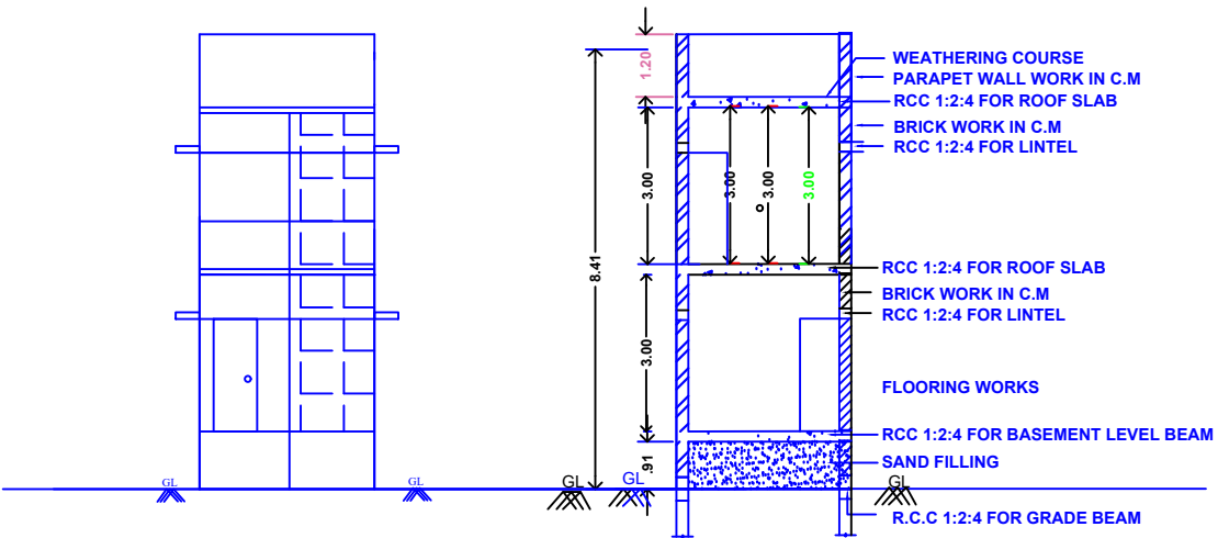
FRONT ELEVATION
