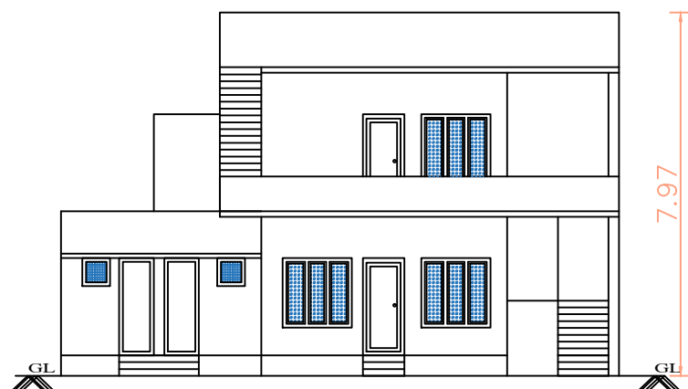
FRONT ELEVATION
