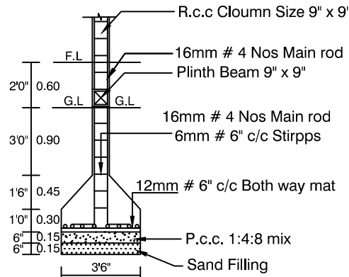
COLUMN DETIAL NOT TO SCALE
