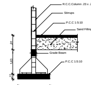
COLUMN DETAIL
