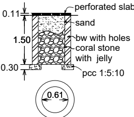
percolation pit
