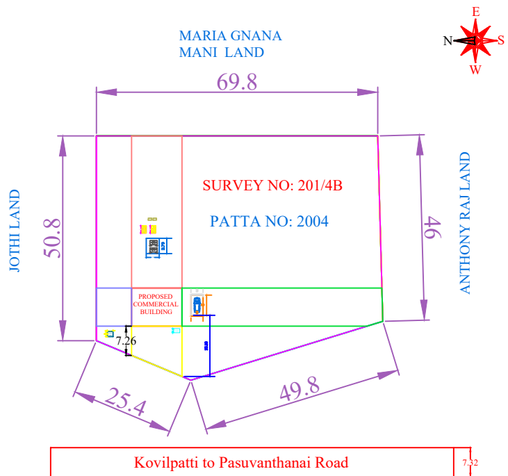
SITE PLAN
