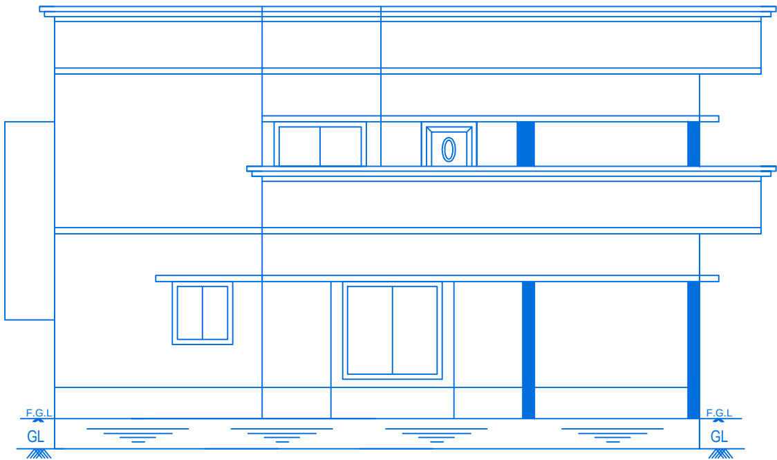
FRONT ELEVATION
