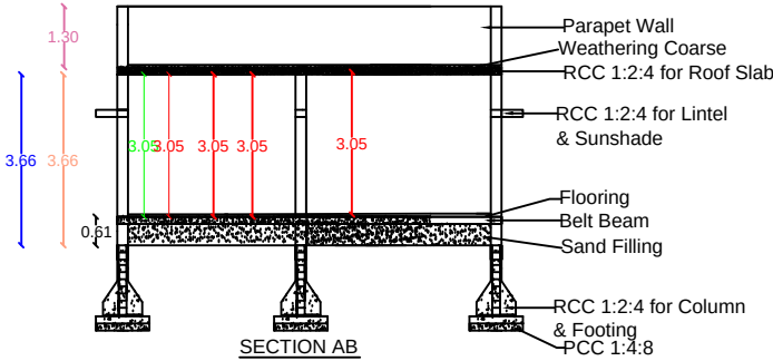
SECTION AB
