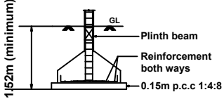
TYP.DET.COLUMN FOOTING
