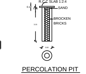
PERCOLATION PIT
