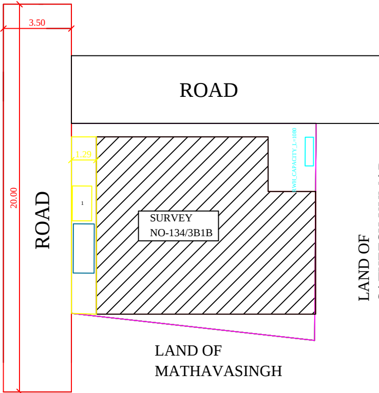
SITE PLAN
