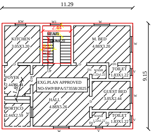
EXG.GROUND FLOOR PLAN
