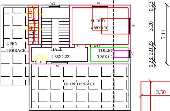
PRO.FIRST FLOOR PLAN
