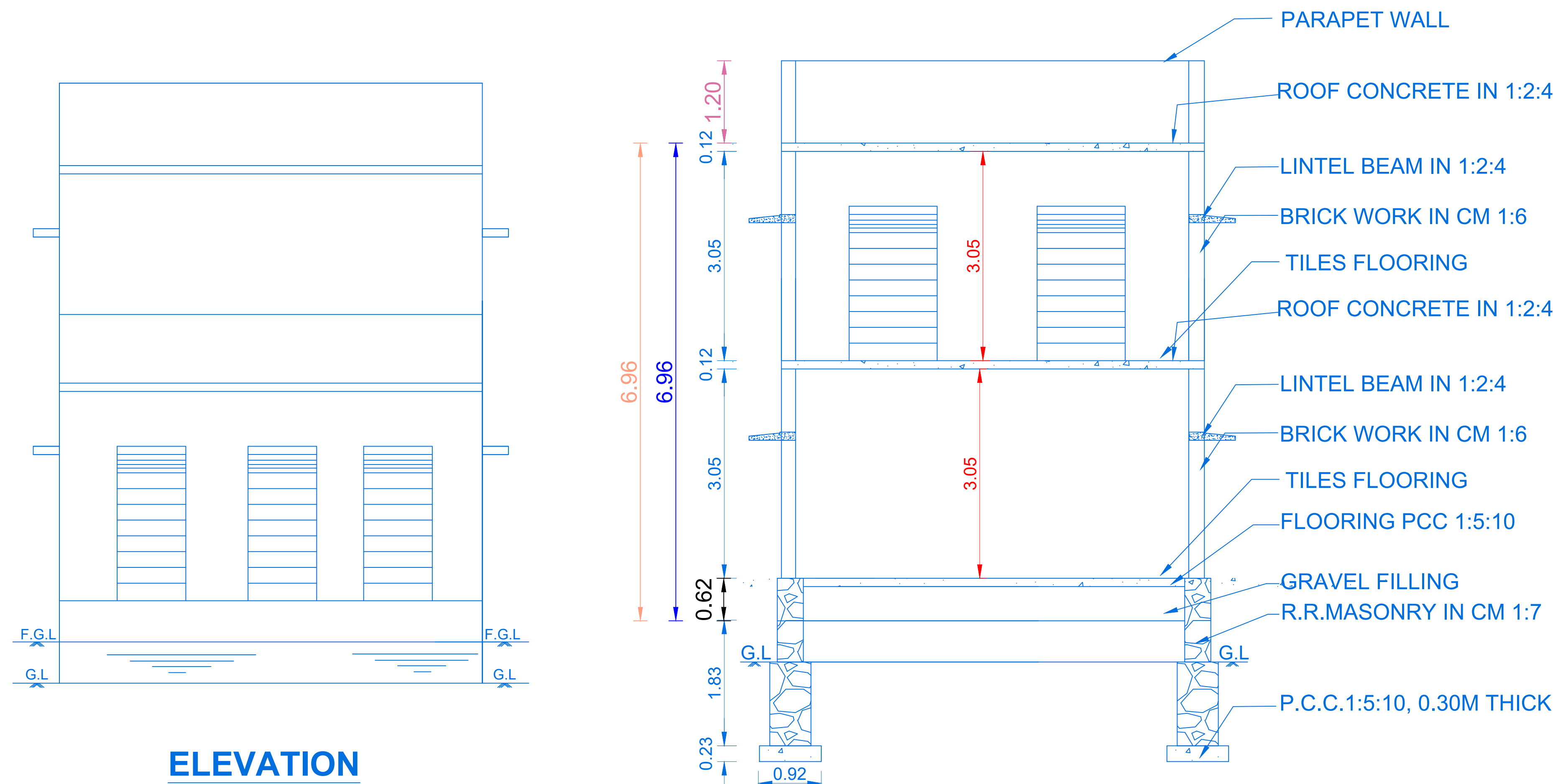
SECTION ON - AA
