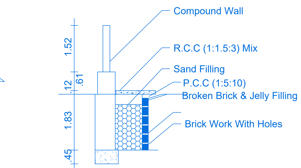
RAIN WATER HARVEST DETAILS
