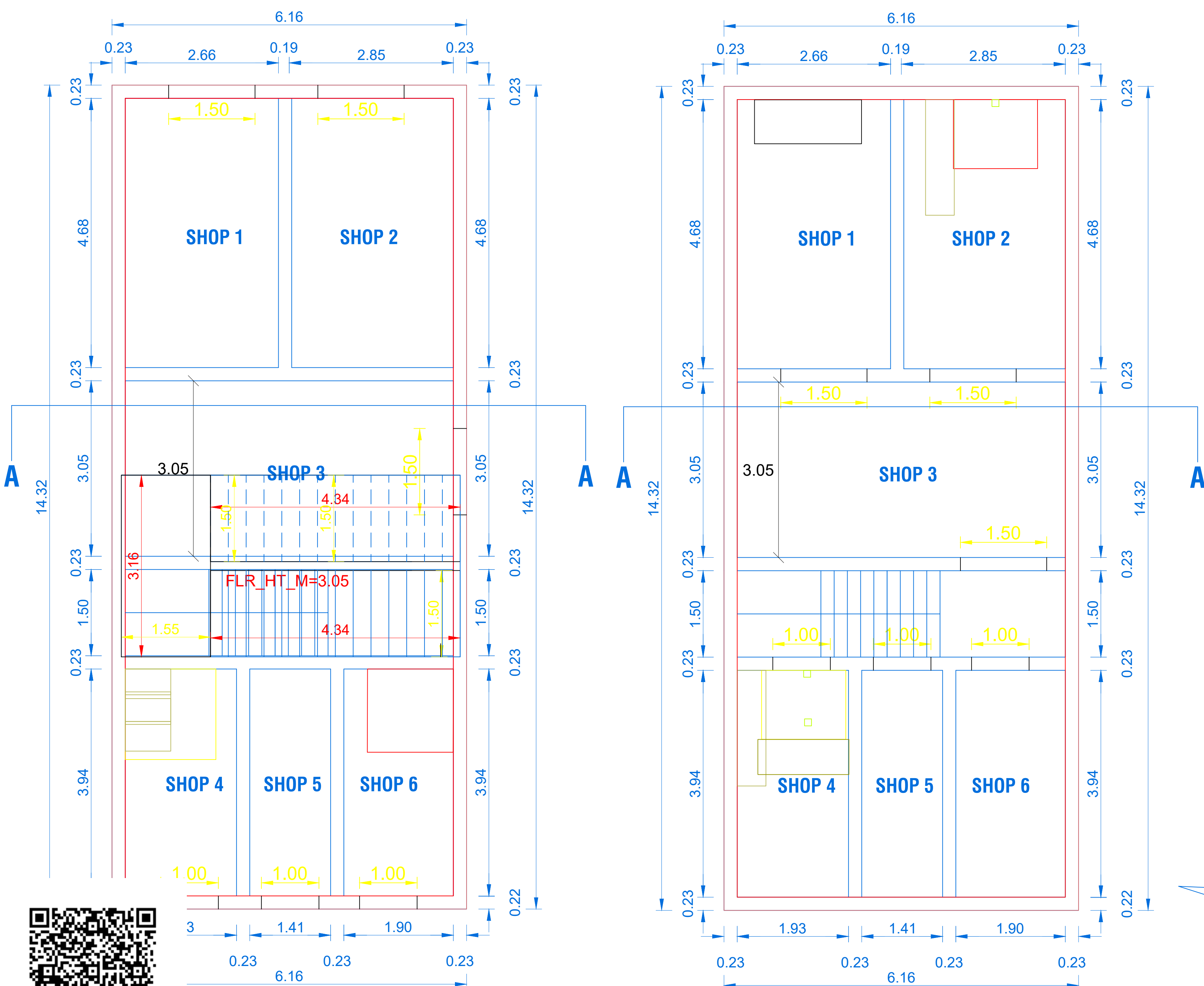
JND FLOOR PLAN
