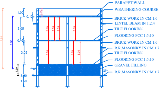
SECTION ON "V-B"
