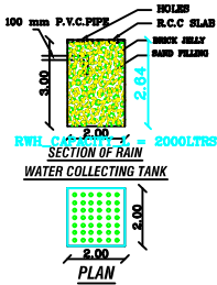
PLAN
