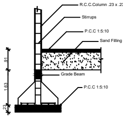
COLUMN DETAIL
