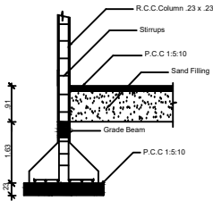
COLUMN DETAIL
