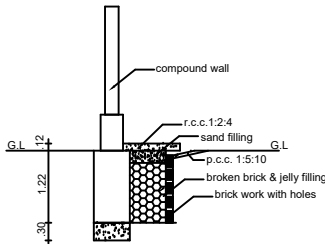
PLINTH BOUNDARY PERCOLATION PIT
