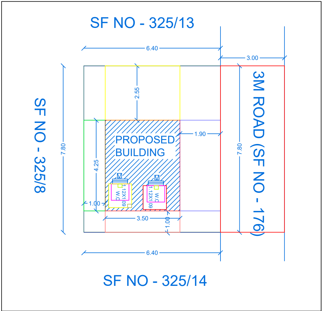
SITE PLAN
