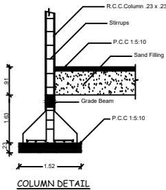
COLUMN DETAIL
