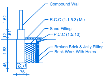
RAIN WATER HARVEST DETAILS
