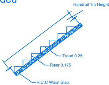
STAIR DETAILS
