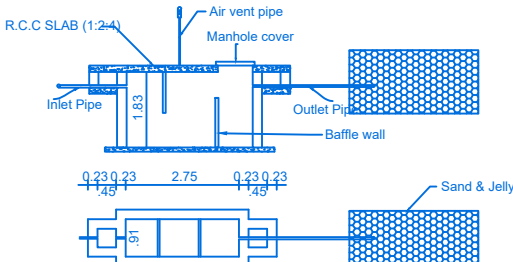
SEPTIC TANK & TRENCH
