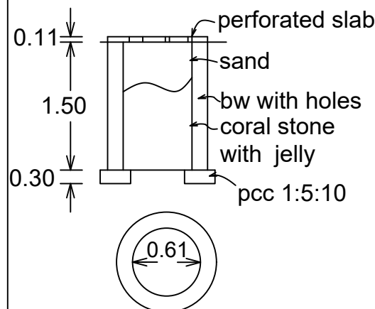
percolation pit
