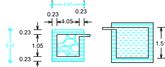
RWH_CAPACITY_L=1000LTRS DETAILS OF FILTER BED & WELL
