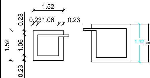
RWH_CAPACITY_L=2000L RAIN WATER HARVESTING
