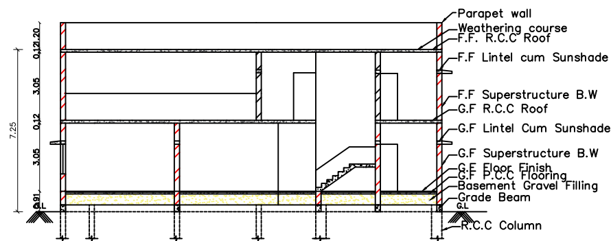
CROSS SECTION ON BB
