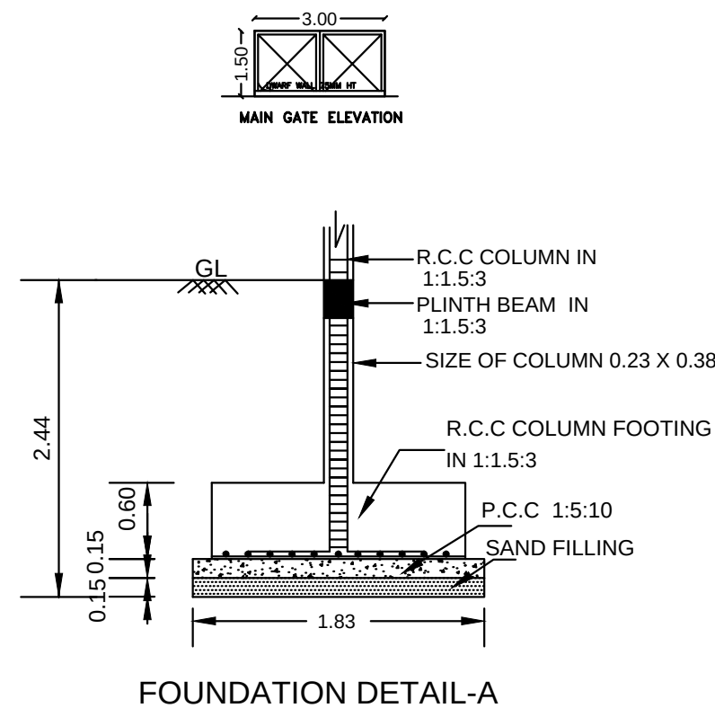
FOUNDATION DETAIL-A
