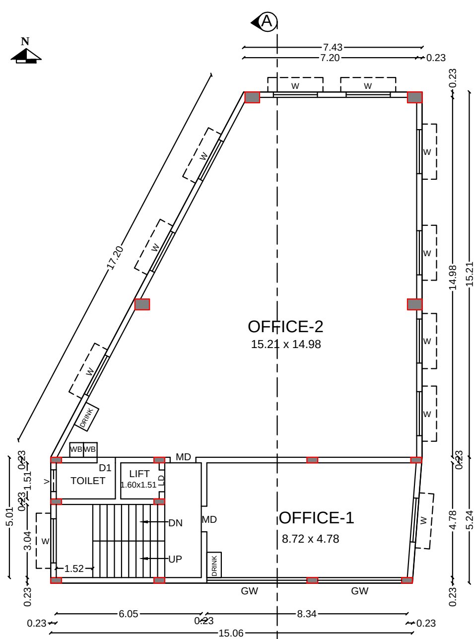
TYPICAL FLOOR PLAN (1ST & 2ND FLOORS)
