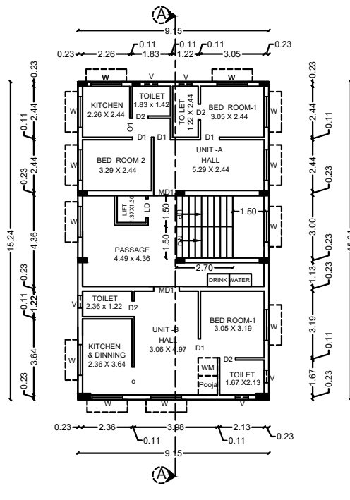
TYPICAL FLOOR PLAN (1ST, 2ND & 3RD FLOORS)
