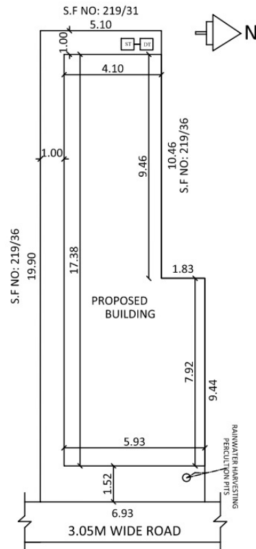
SITE PLAN
