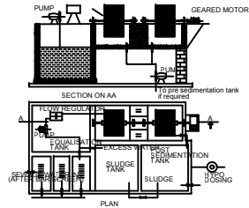
SEWAGE TREATMENT PLANT DETAILS
