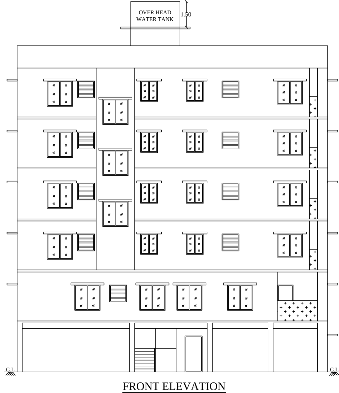
FRONT ELEVATION
