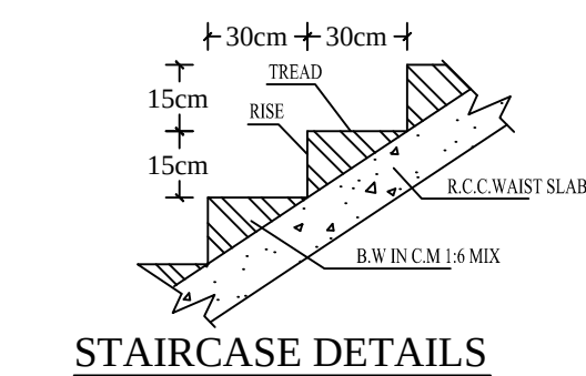
STAIRCASE DETAILS
