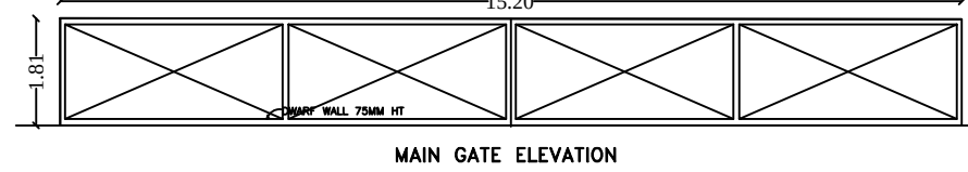
MAIN GATE ELEVATION
