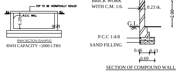
SECTION OF COMPOUND WALL
