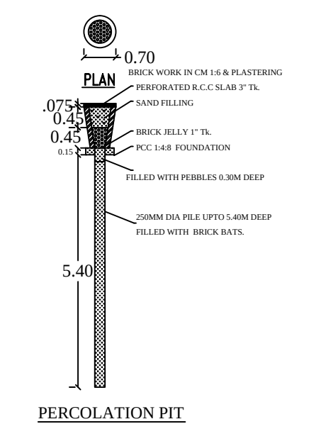
PERCOLATION PIT
