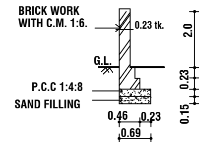
SECTION OF COMPOUND WALL
