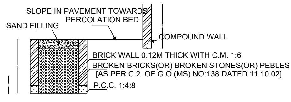
SECTION OF RAIN WATER PERCOLATION BED RWH_CAPACITY_L=5000LTRS
