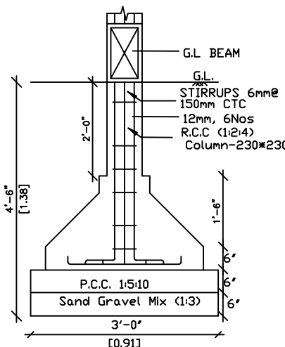
R.C.C. COLUMN FOOTING DETAILS
