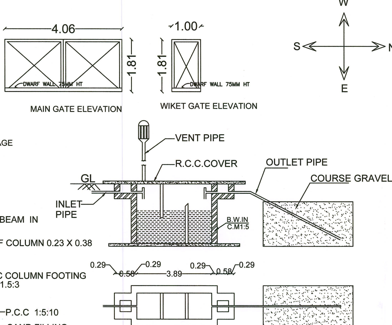
SEPTIC TANK & DISPERSION TRENCH DETAILS
