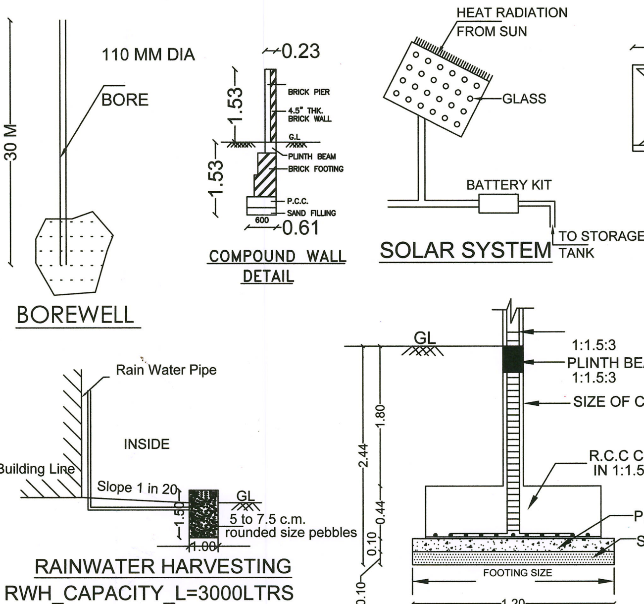
FOUNDATION DETAILS
